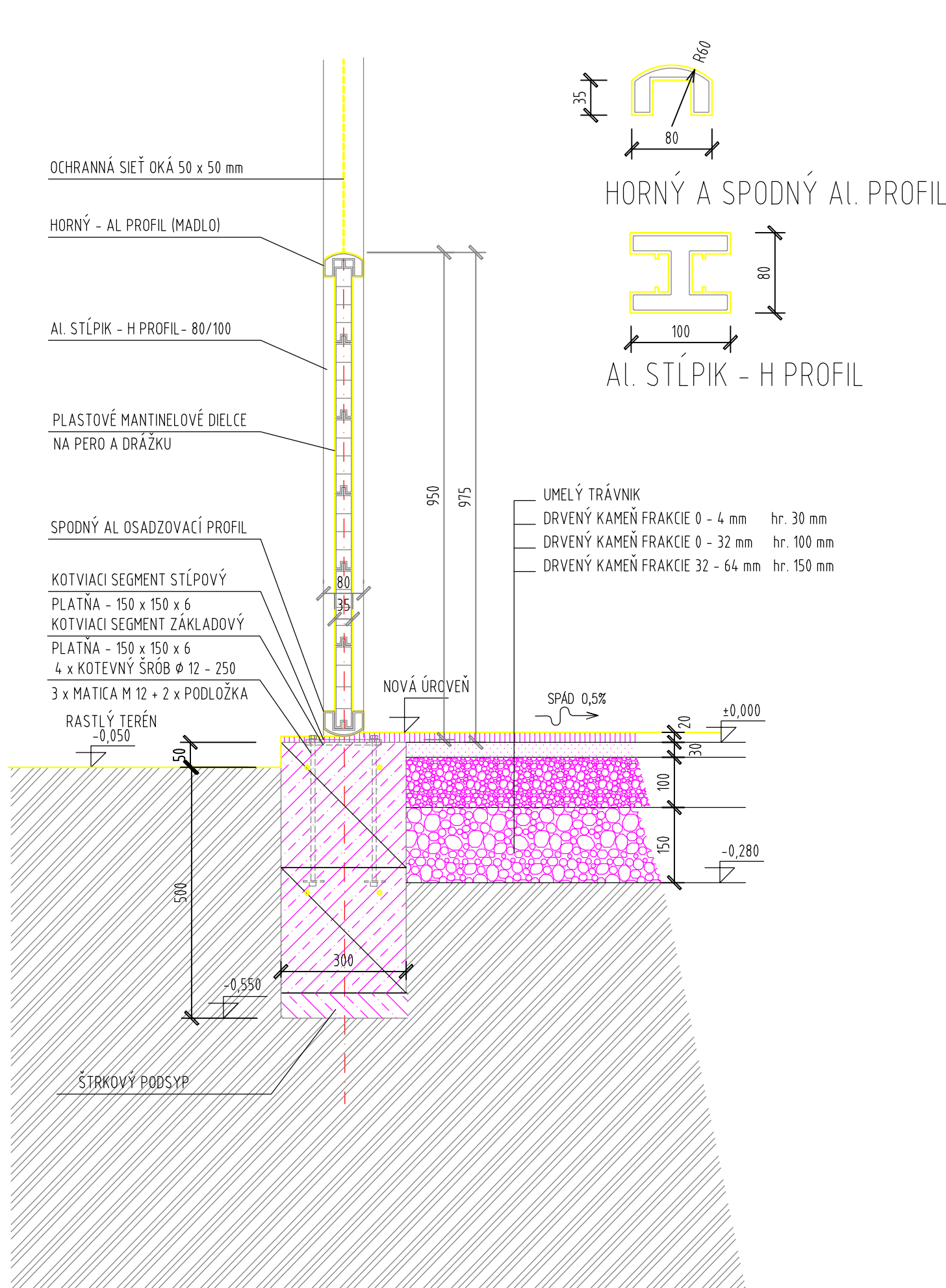
Detail mantinelu - m 1:10
